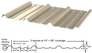
PBR 36" Coverage
