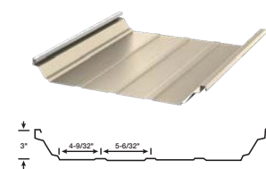
TS-324 24" Coverage
