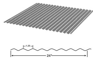
Corrugated 24" Coverage
