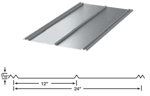
5-V 24" Coverage
