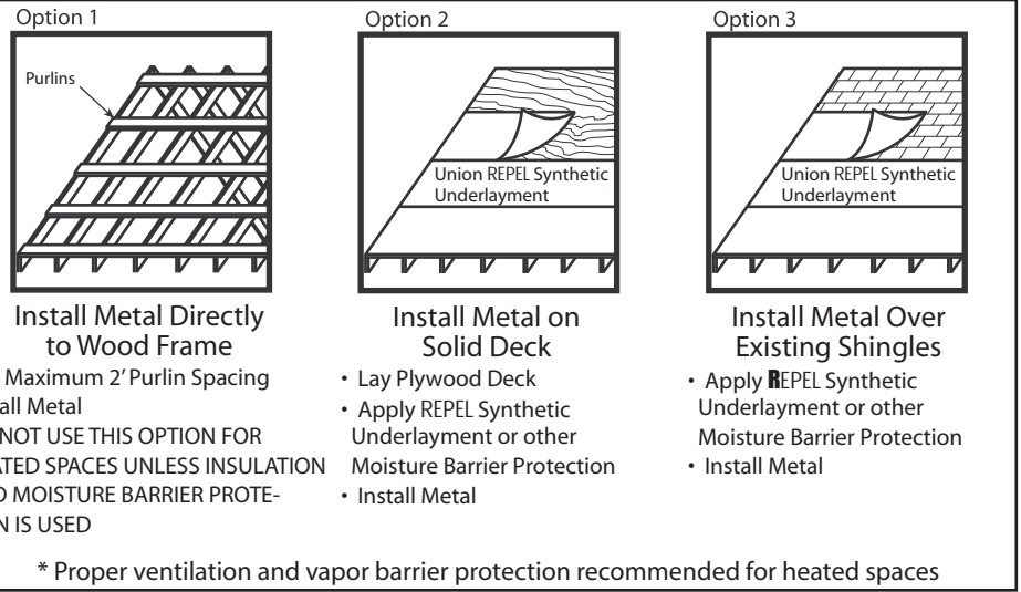
Figure 5 - Installation Options
